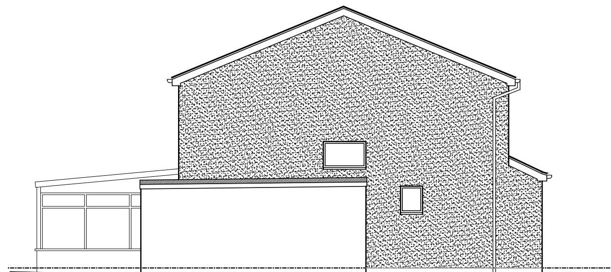
SIDE ELEVATION
