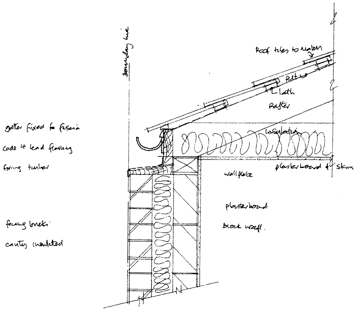
TYPICAL DETAIL AT BOUNDARY (1:10 Scale)
