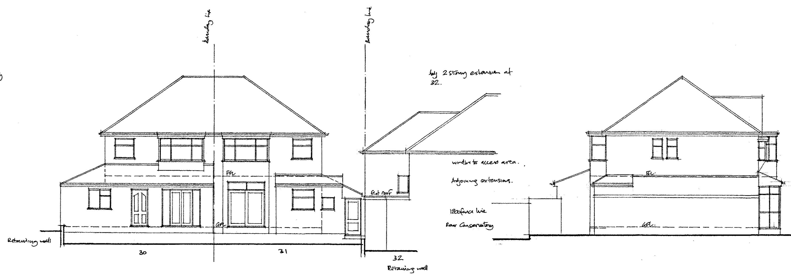
REAR ELEVATION
