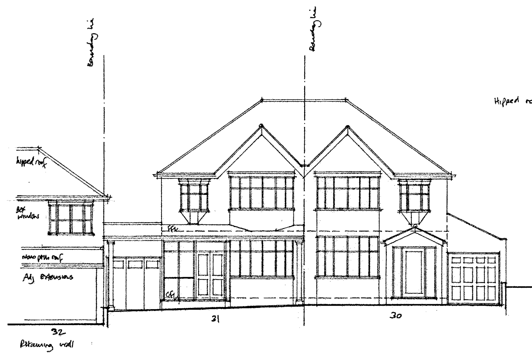
FRONT ELEVATION
