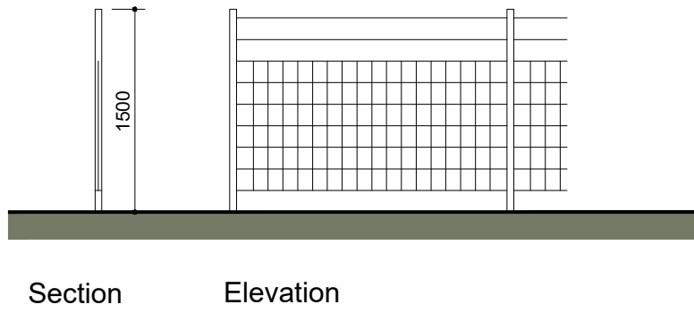
1.5m high timber post & wire fence
