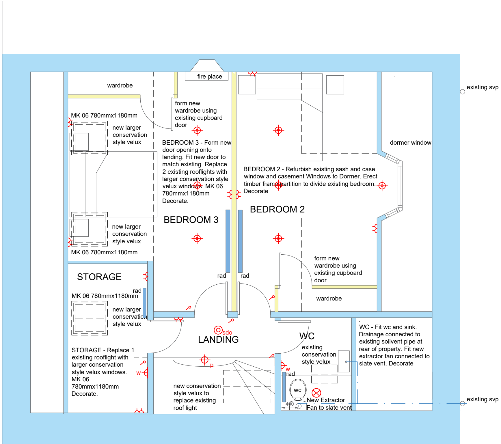
PROPOSED ATTIC PLAN
