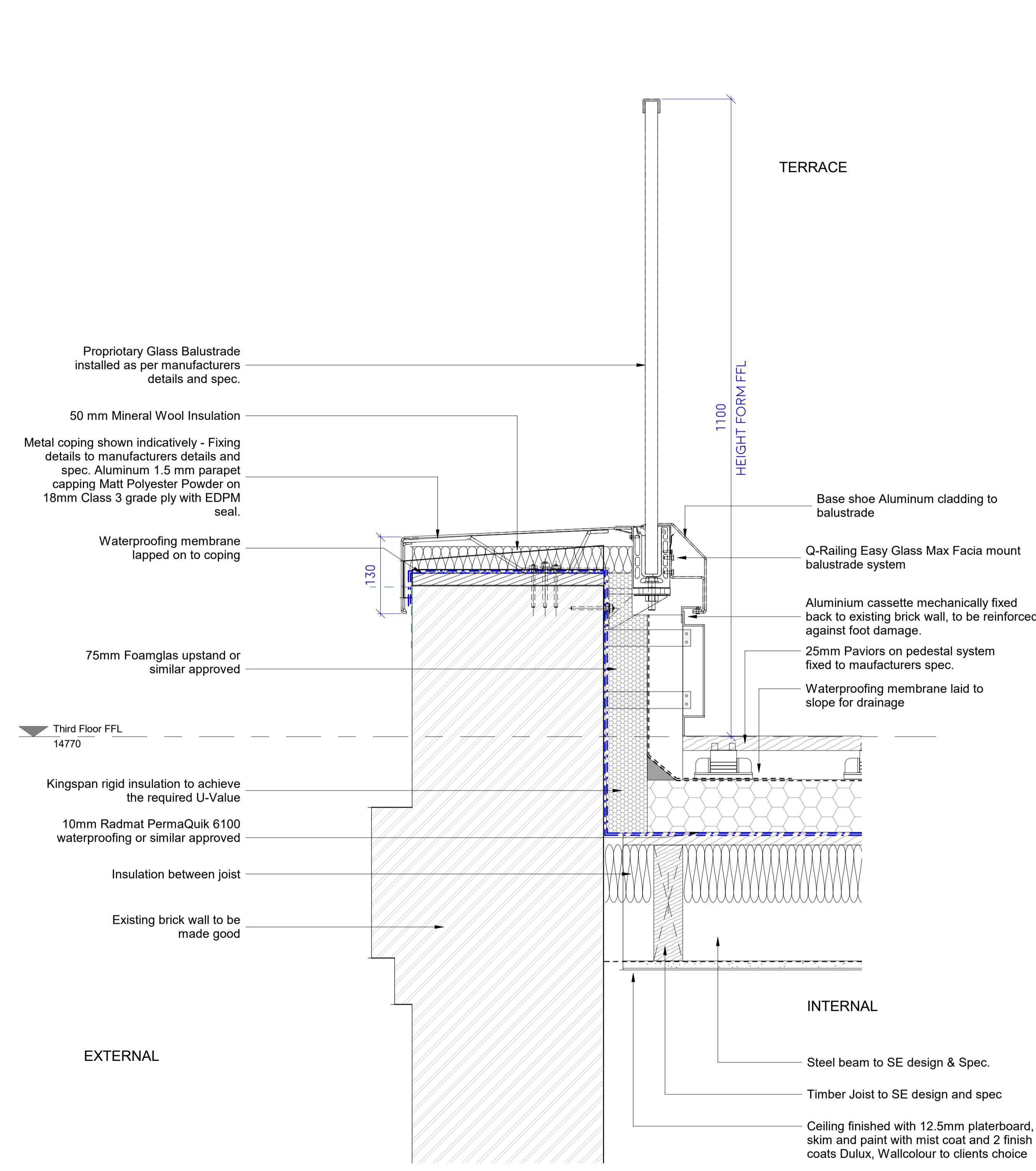
1 Wall to New Balcony Junction 1:5
