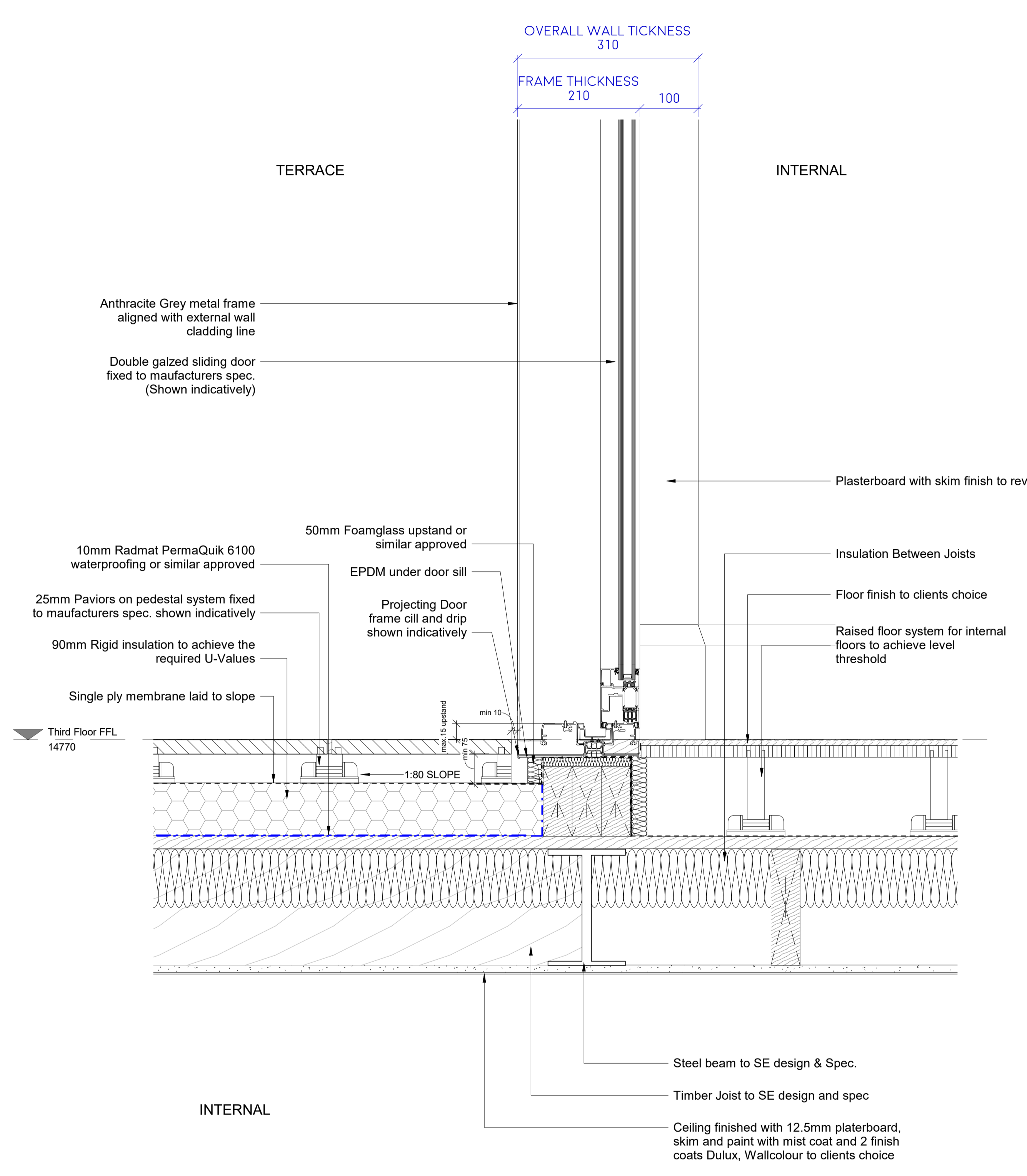
2 New Balcony to New Wall Junction 1:5
