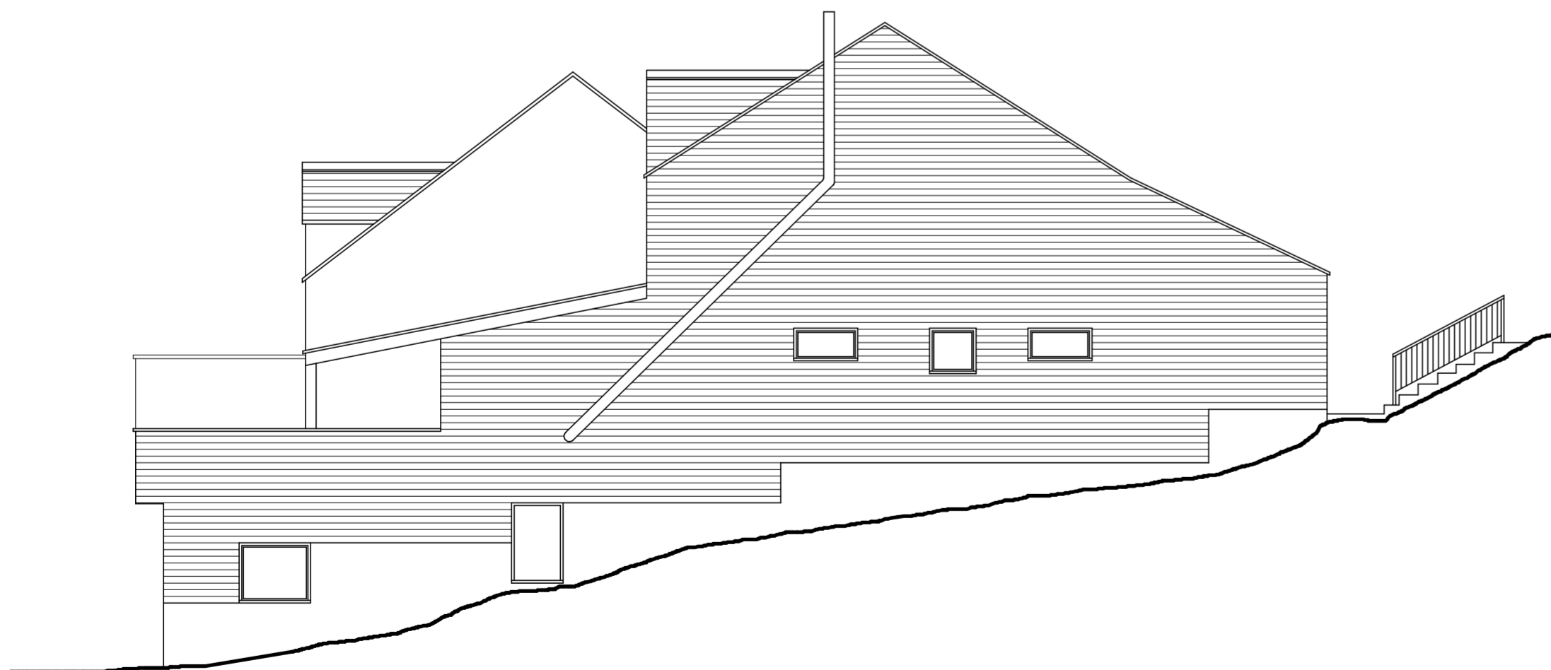
south elevation
