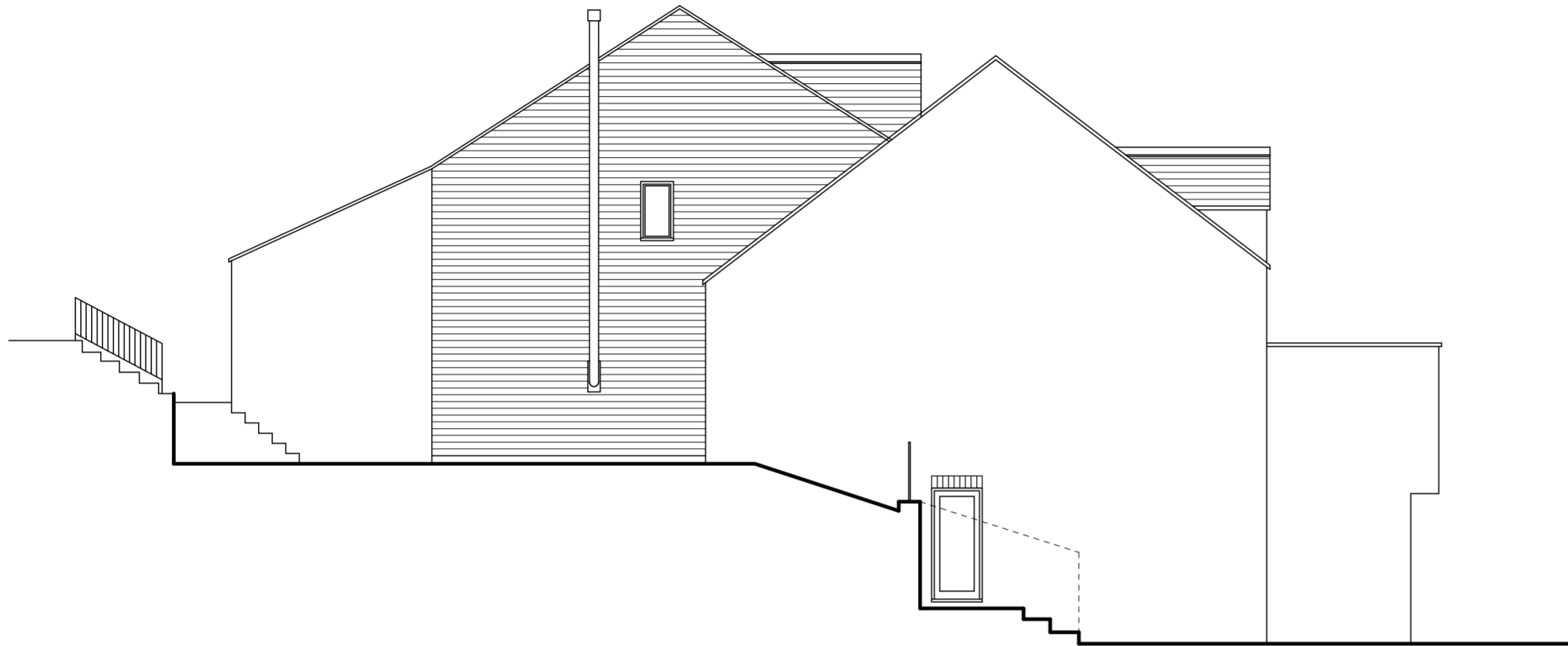
NORTRH ELEVATION
