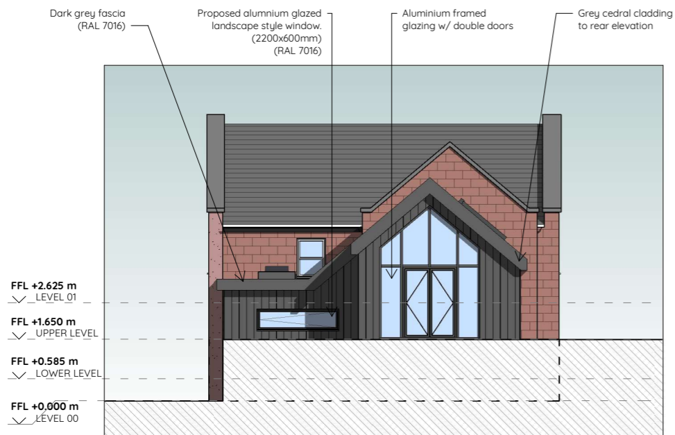
1 EAST ELEVATION - AS PROPOSED 1:100
