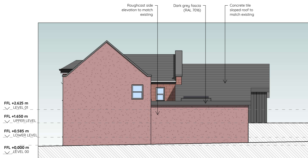
3 SOUTH ELEVATION - AS PROPOSED 1:100
