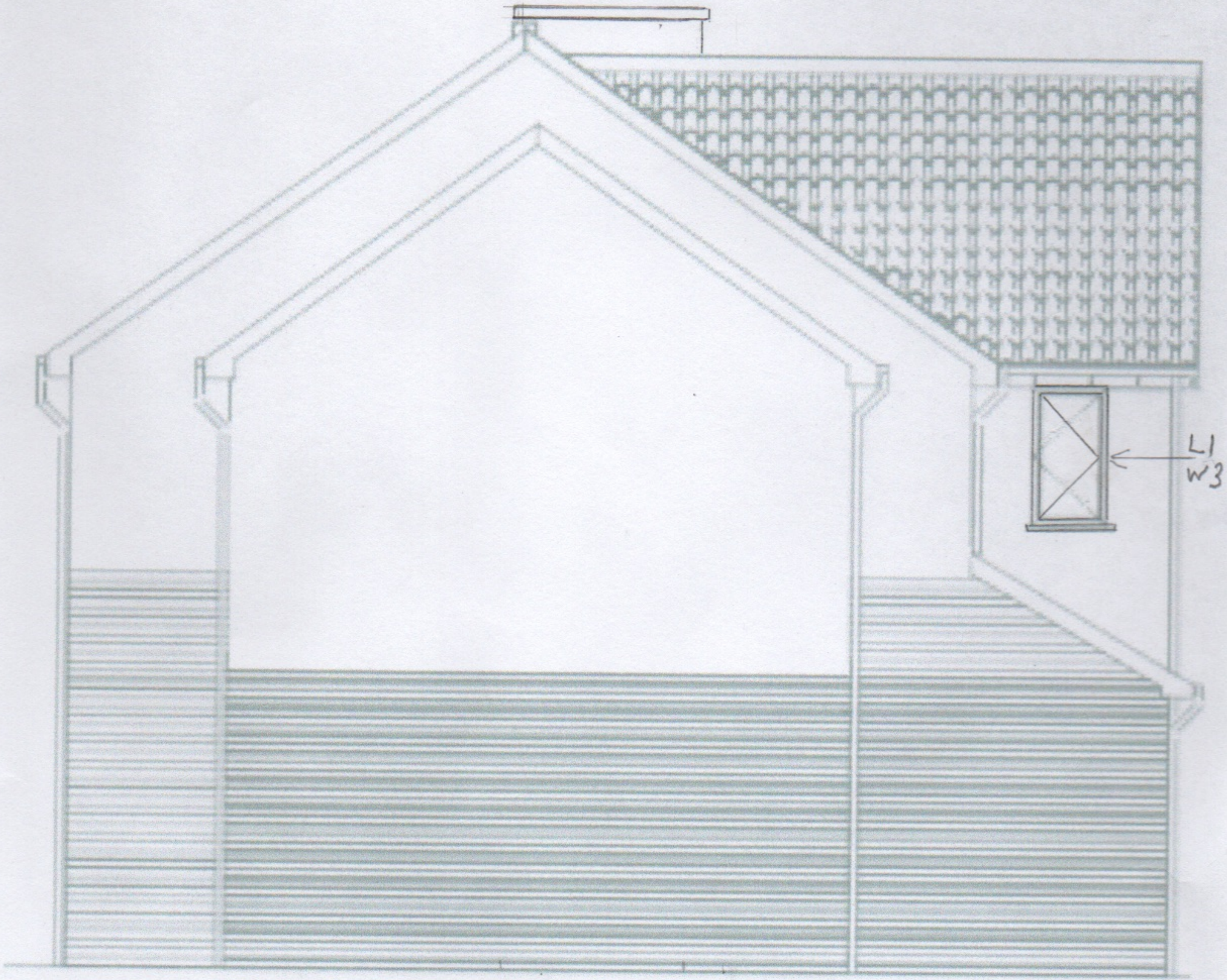
PROPOSED EAST FACING SIDE ELEVATION SCALE 1:50
