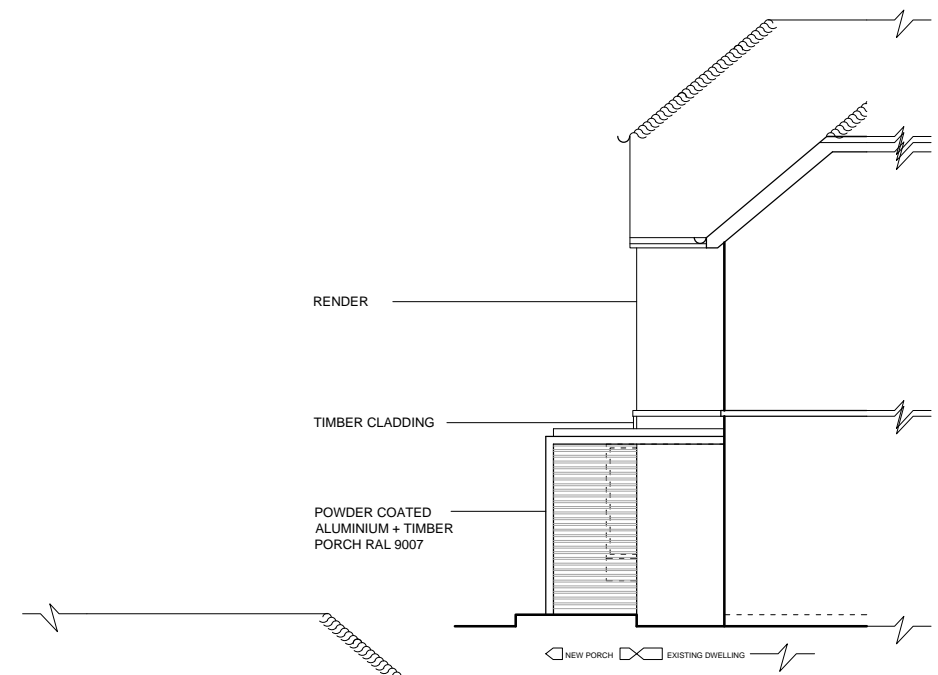
PARTIAL NW ELEVATION
