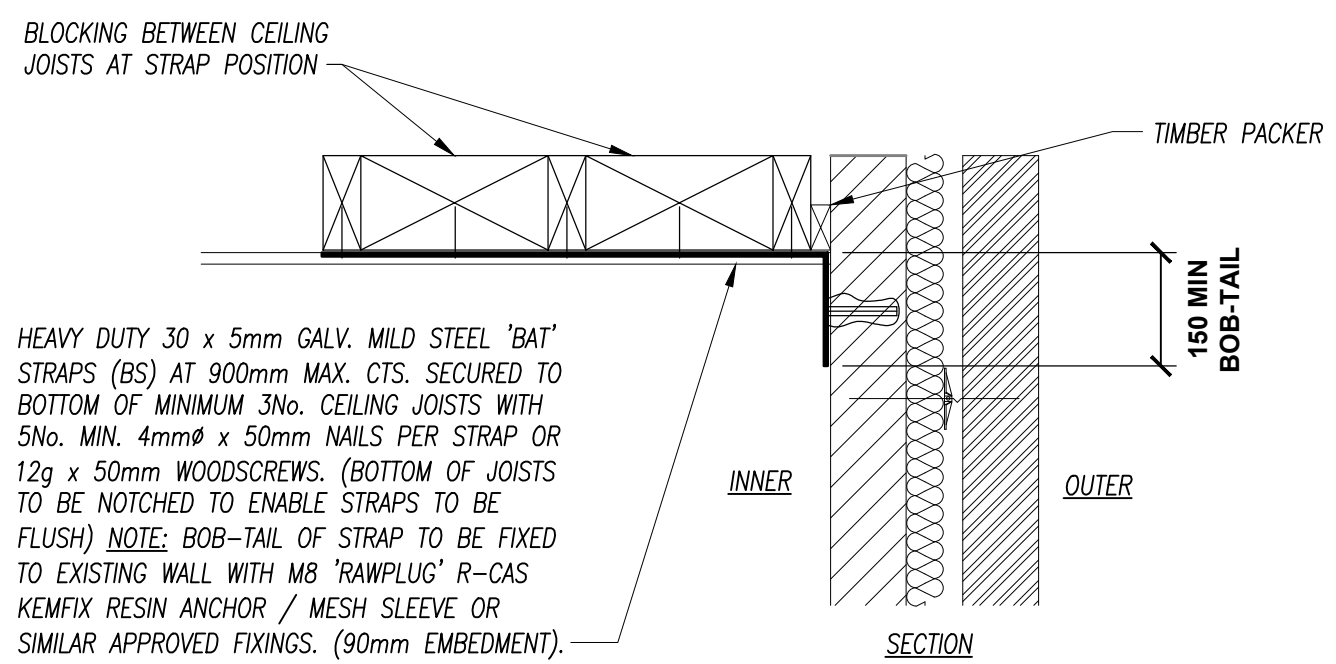
TYPICAL WALL RESTRAINT DETAIL AT CEILING LEVEL (1:10)
