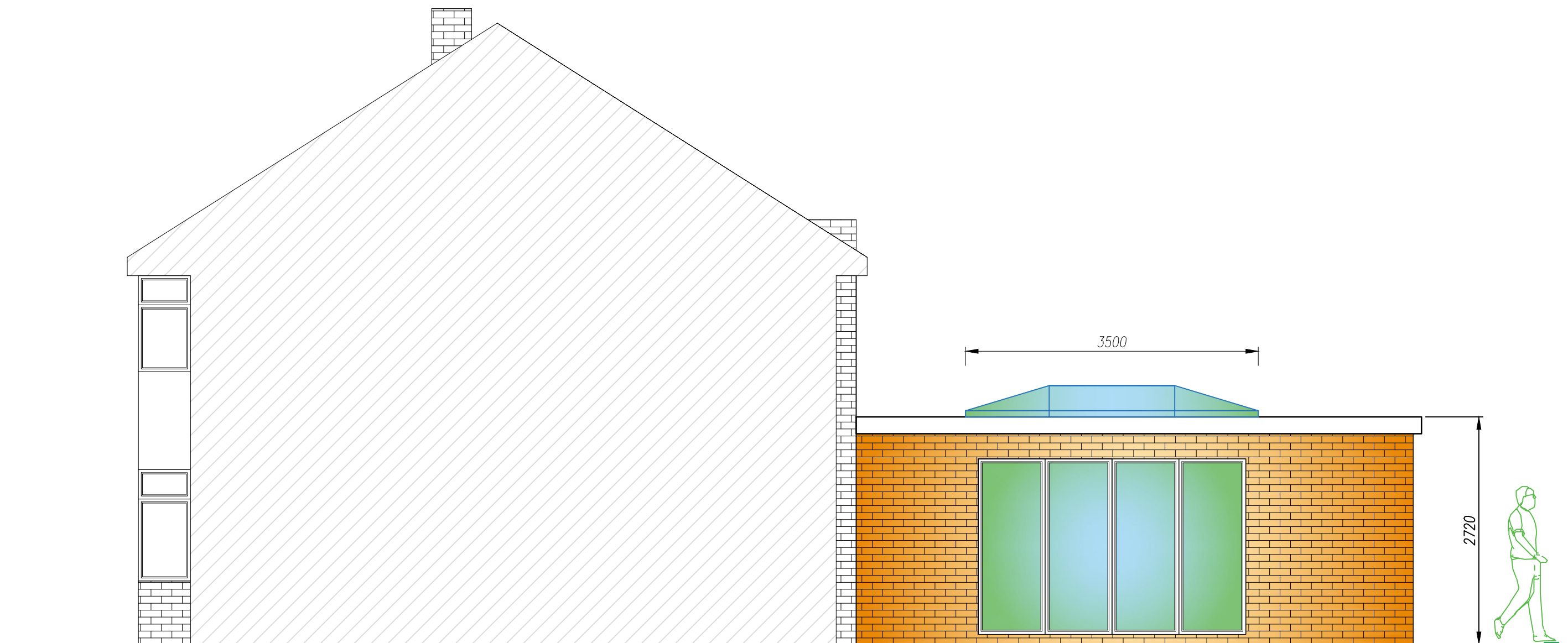
PROPOSED RIGHT SIDE ELEVATION (1:50)
