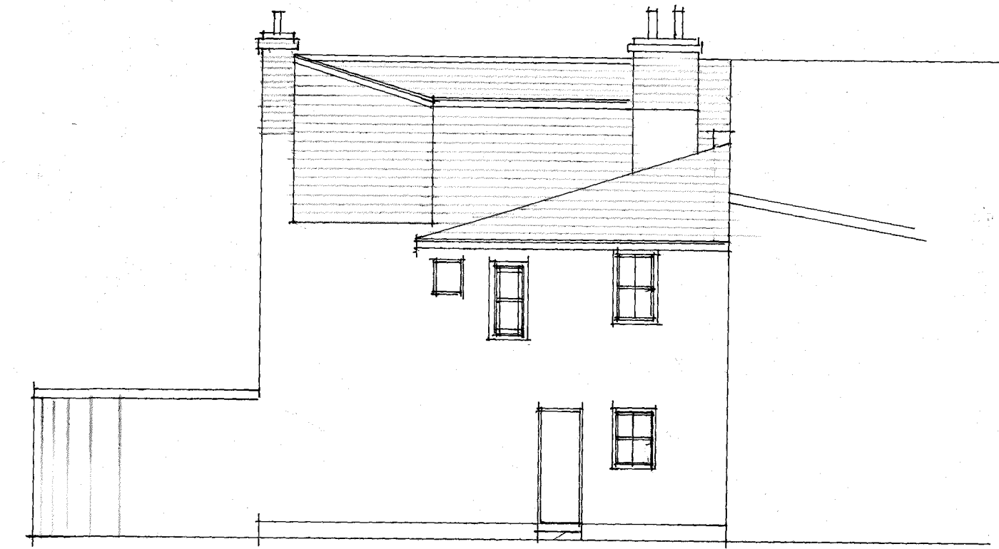
nw elevation
