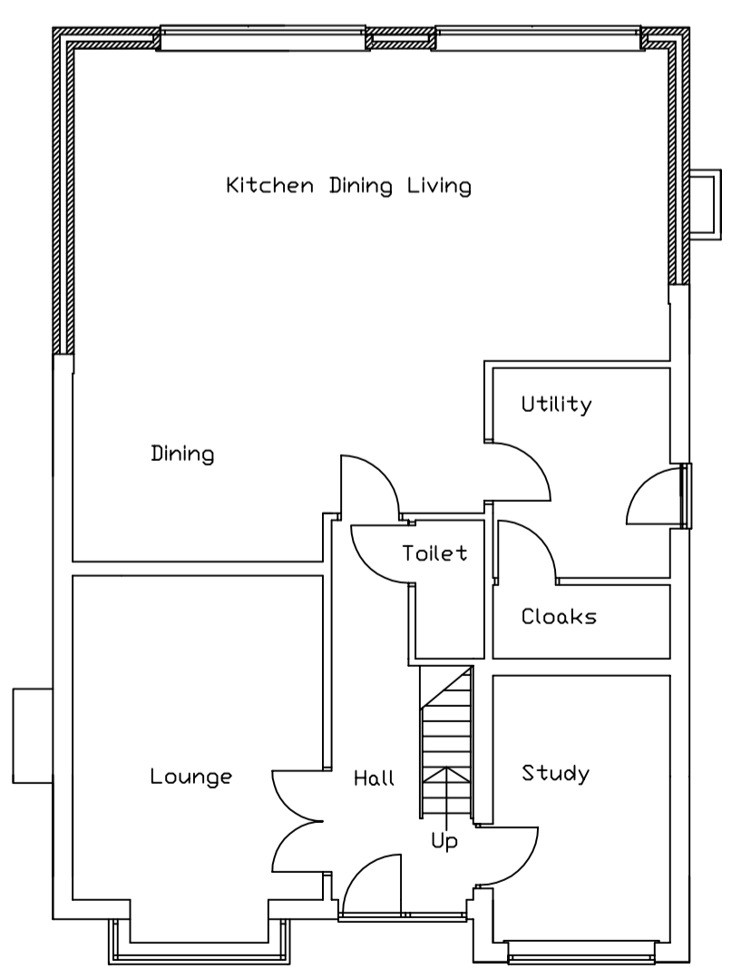
Prop Ground Floor
