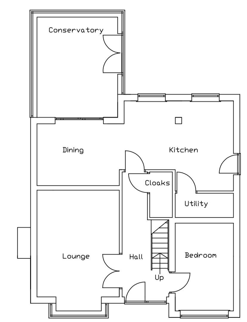
Ex Ground Floor
