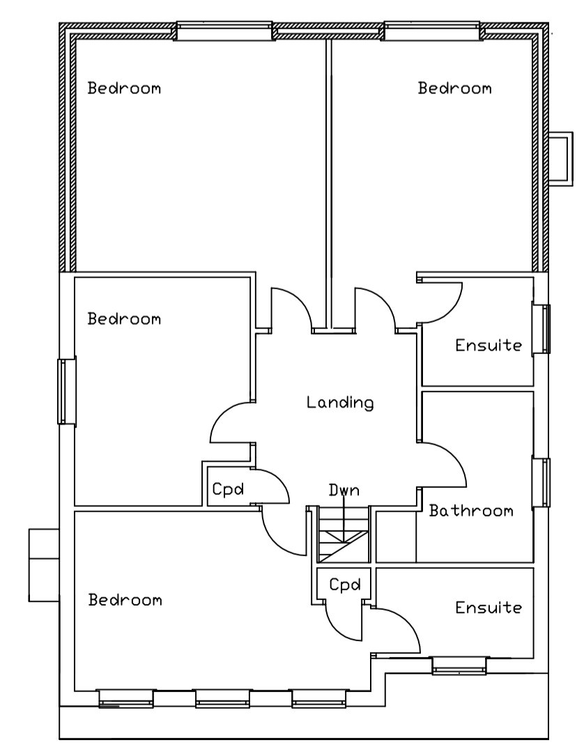
Prop First Floor
