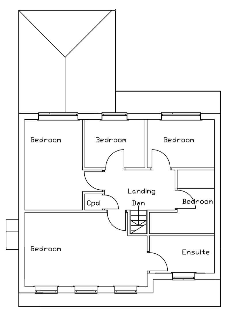
Ex First Floor
