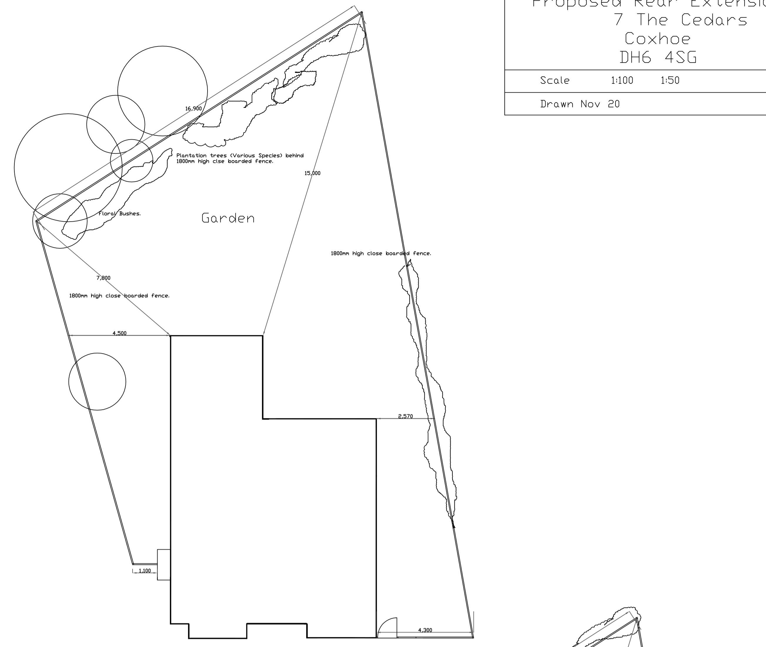
Ex Site Plan
