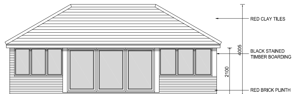
REAR ELEVATION
