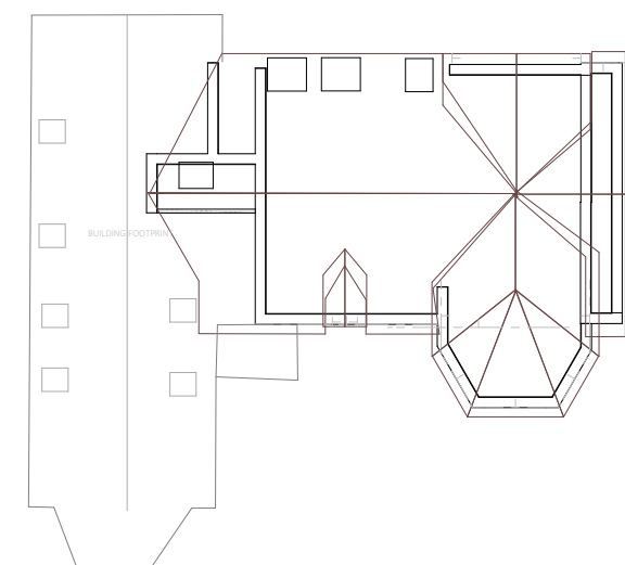
Roof Plan (1:200)
