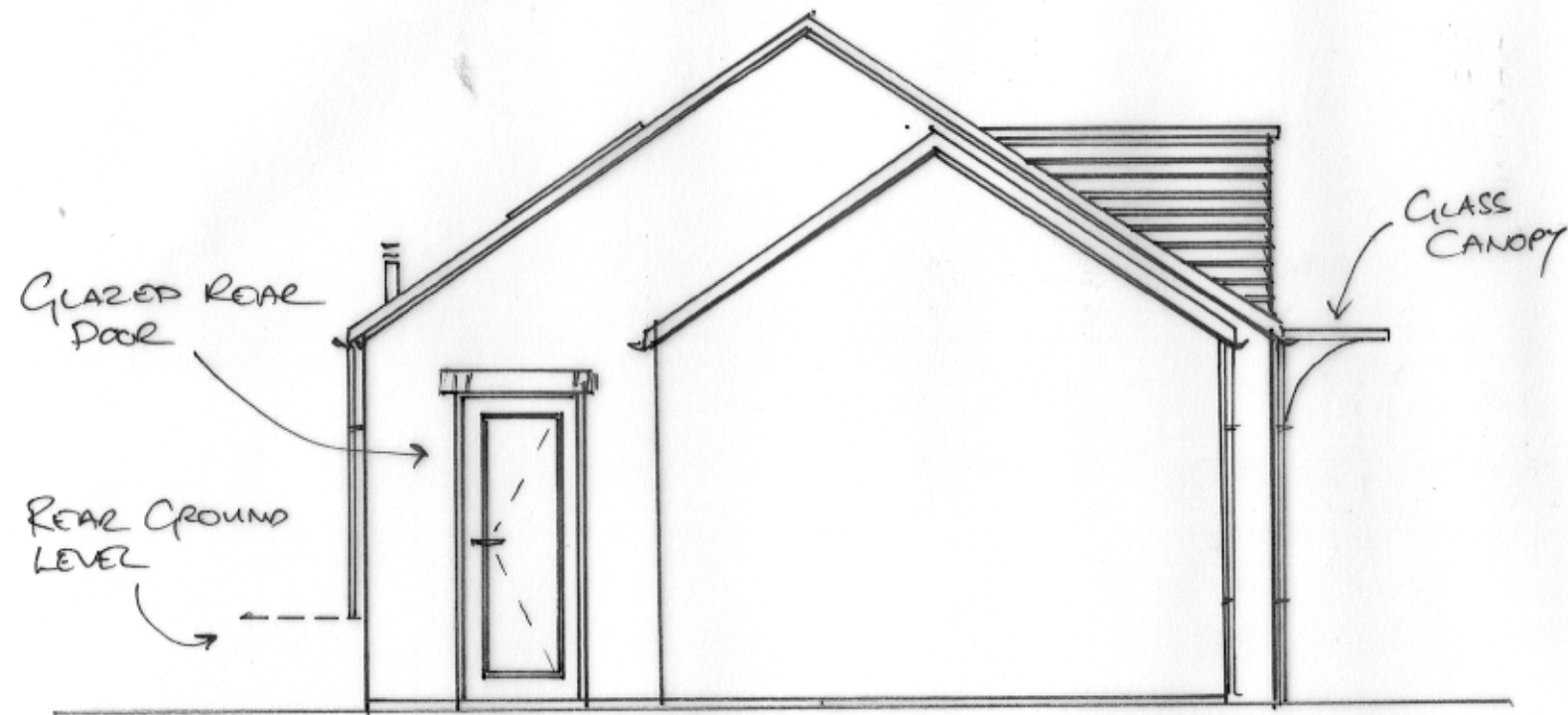
SOUTH ELEVATION
