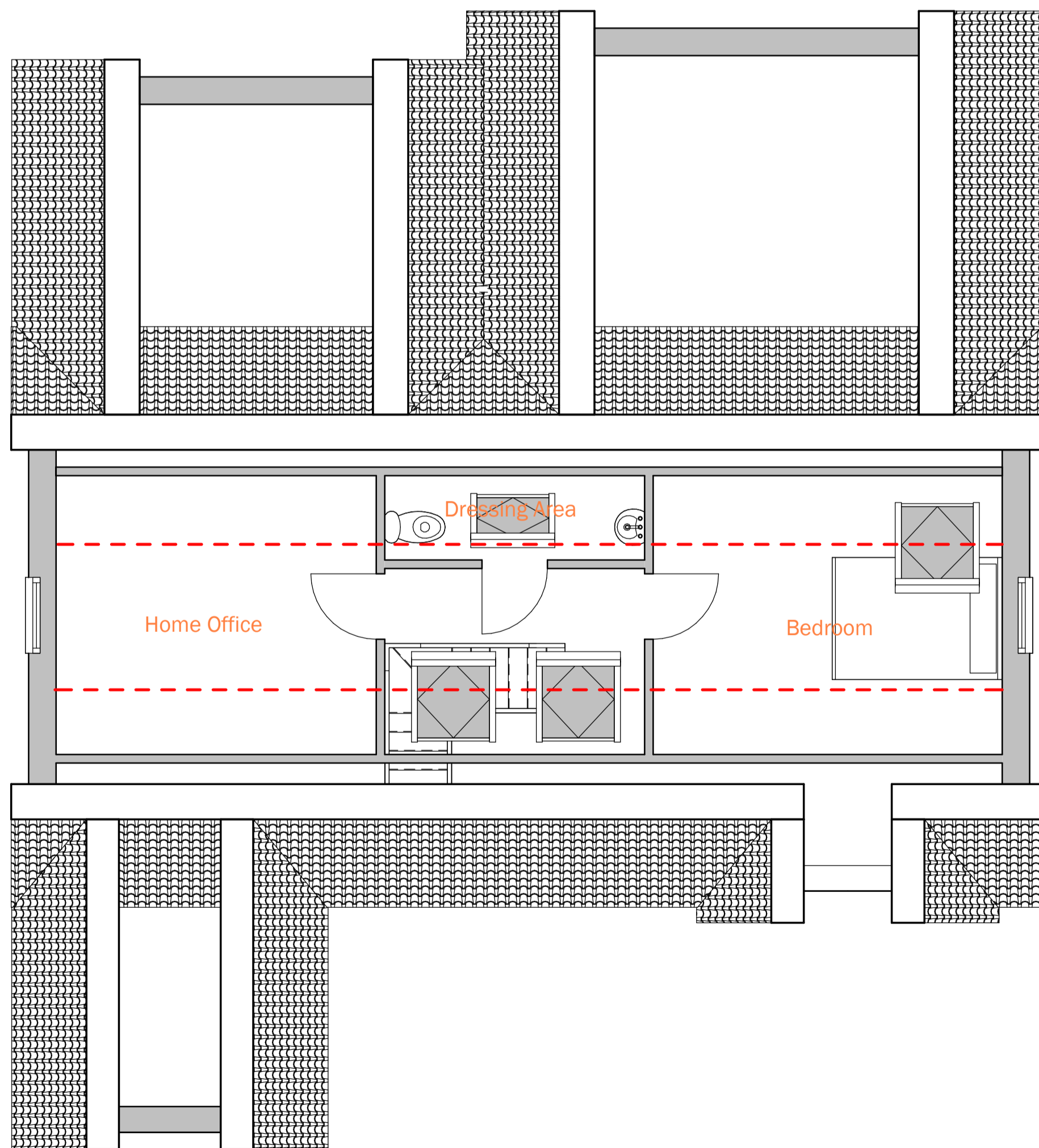
1 SF FFL - PROPOSED 1 : 50
