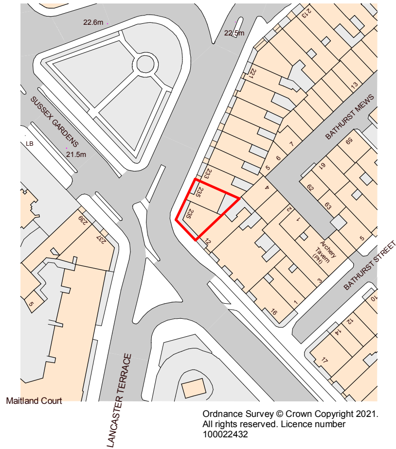
1 Location Plan 1 : 1250
