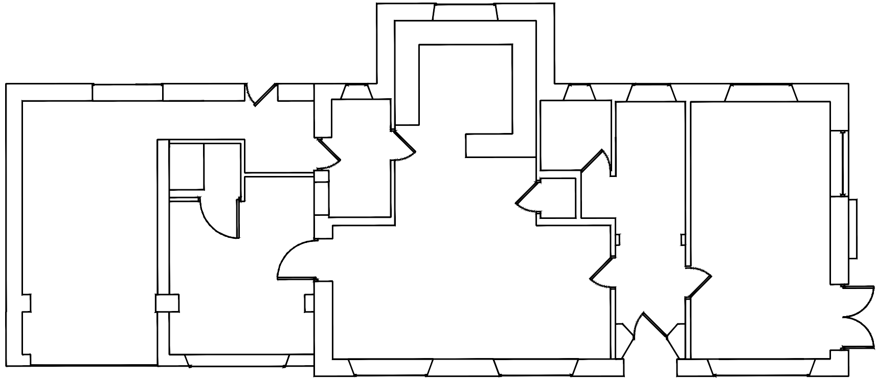
Calluna, Castlett Street, Guiting Power, Cheltenham, Gloucestershire, GL54 5US PROPOSED GROUND FLOOR PLAN
