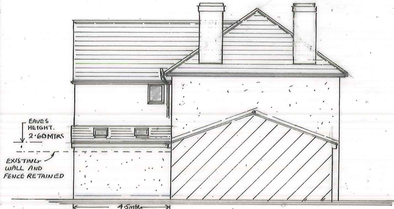
SIDE ELEVATION
