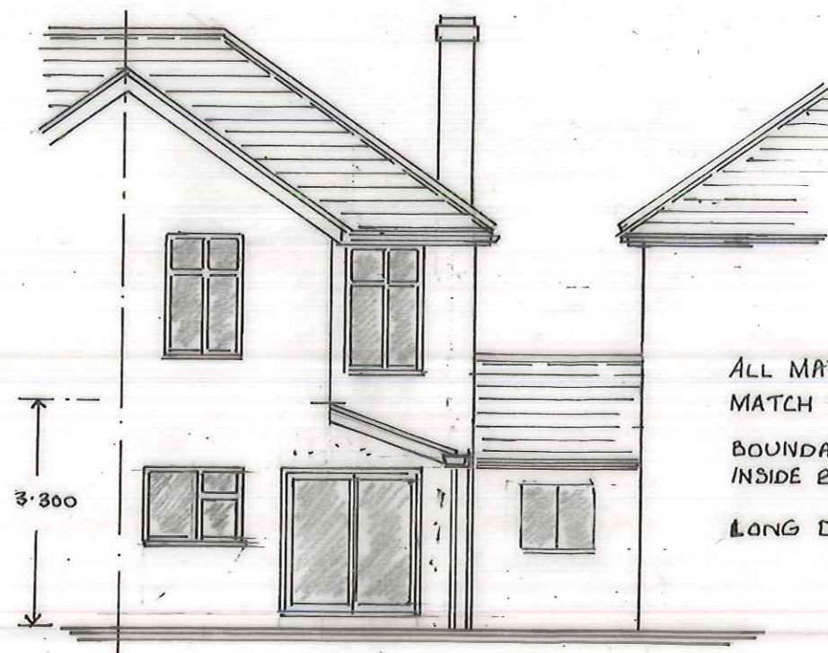
REAR ELEVATION
