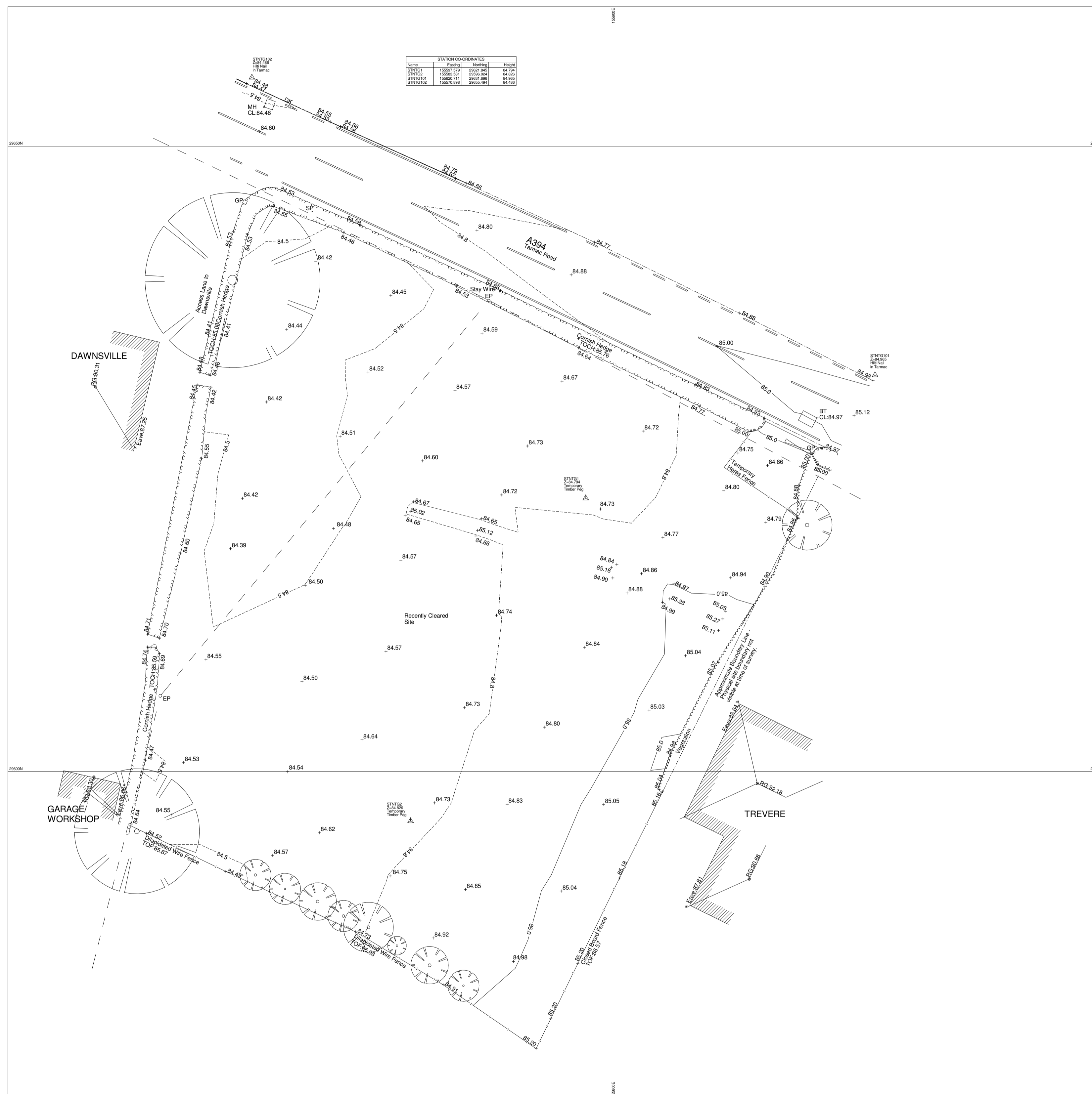
1 Existing Topographical Survey 1 : 200
