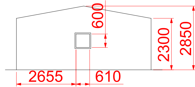
Elevation C
