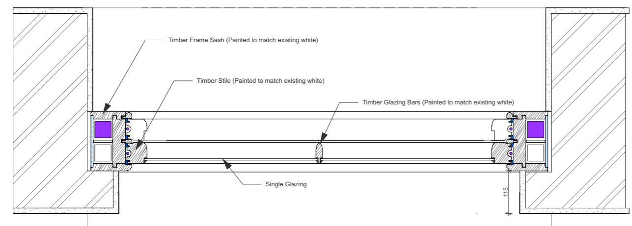
First Floor Window Plan WE-2-03 1:10
