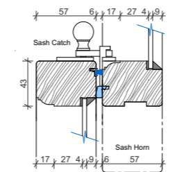
Window Meeting Rail Detail 1:5
