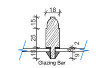
Window Glazing Bar Detail 1:5
