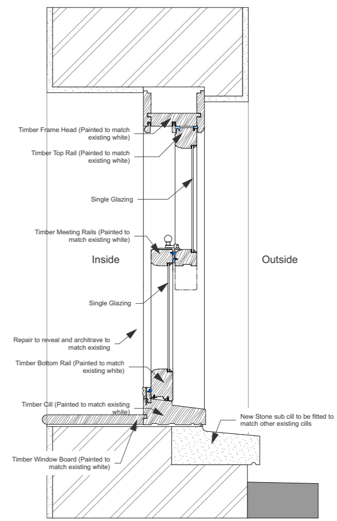
First Floor Window Section WE-2-03 1:10
