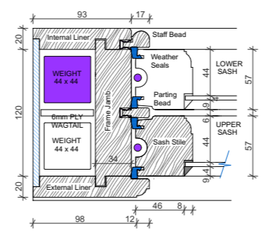
Window Jamb Detail 1:5
