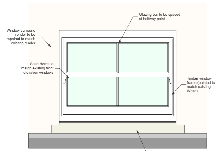
First Floor Window Elevation WE-2-03 1:20
