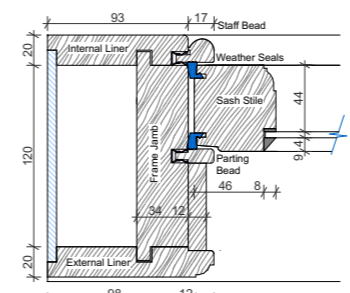
Window Jamb Detail 1:5
