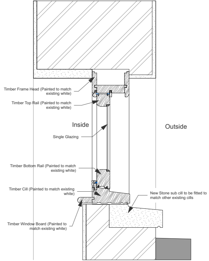
First Floor Window Section WE-2-02 1:10
