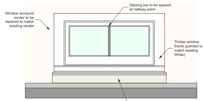
First Floor Window Elevation WE-2-02 1:20
