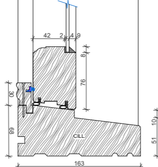
Window Cill Detail 1:5
