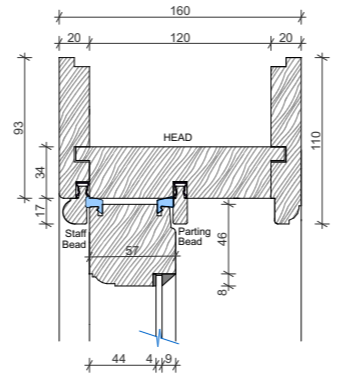
Window Head Detail 1:5
