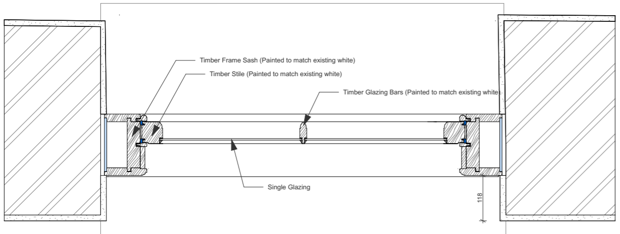
First Floor Window Plan WE-2-02 1:10
