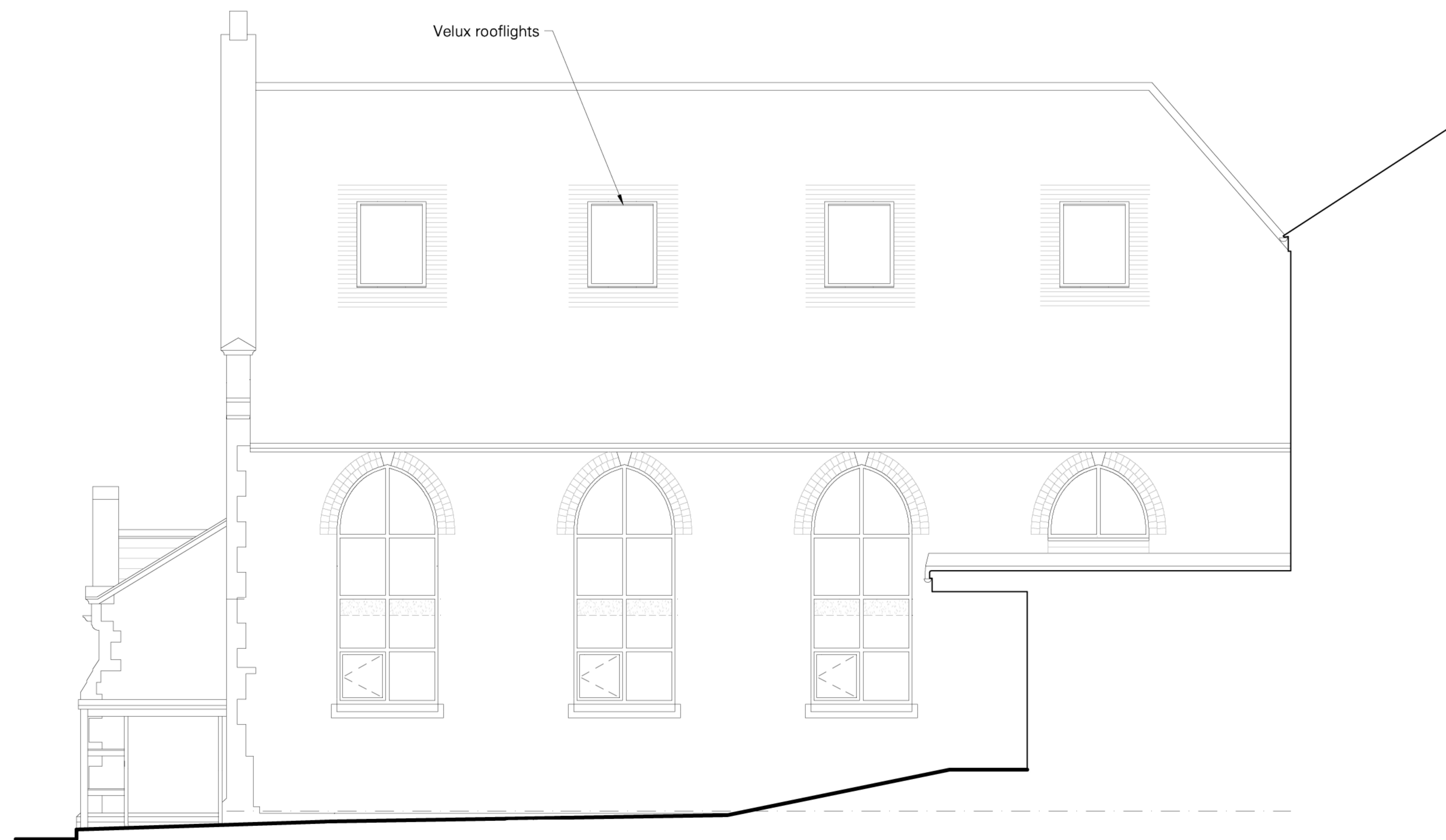
Side/North West Elevation
