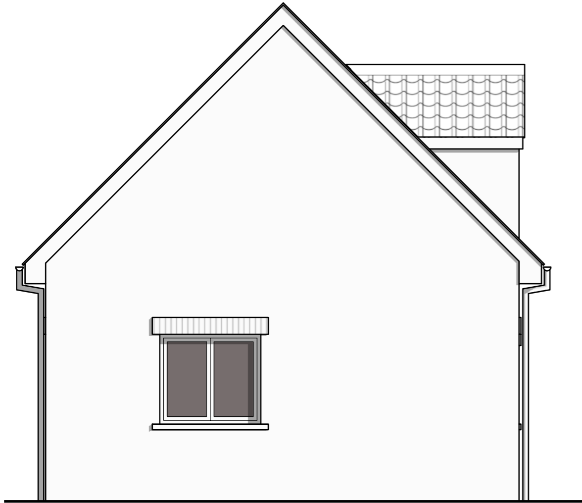
Left (North) elevation
