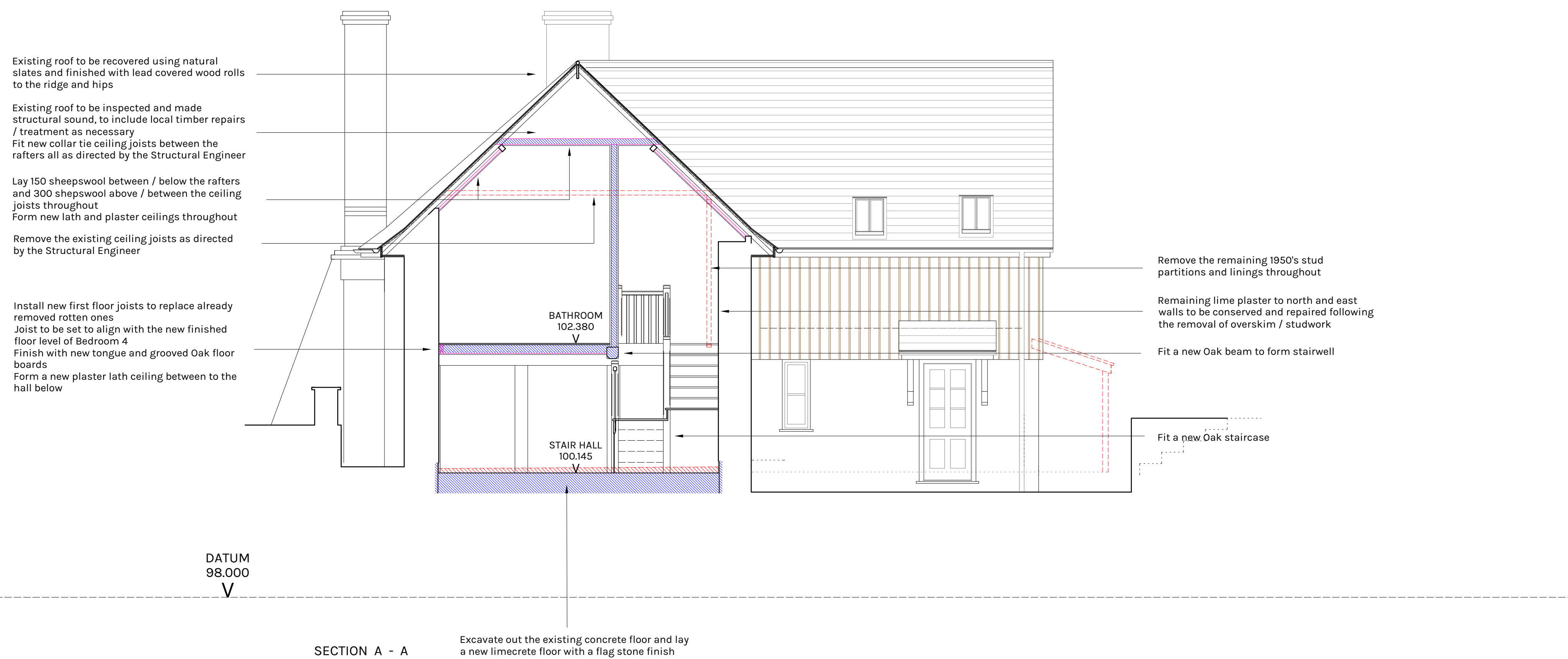
SECTION A - A
