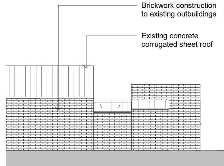
Existing Elevation 3 1 : 100
