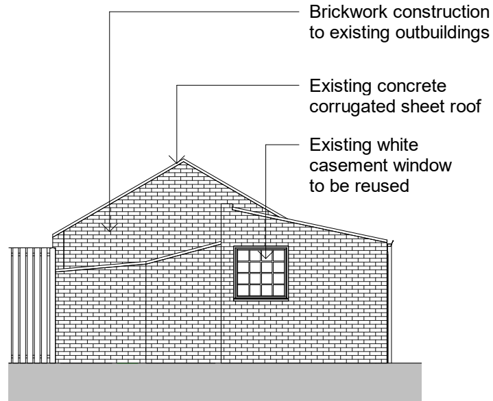
Existing Elevation 2 1 : 100
