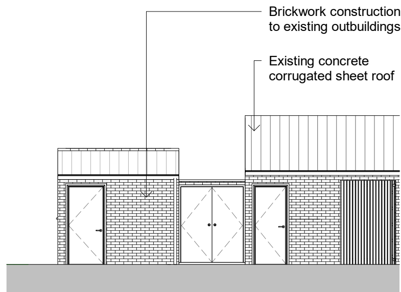
Existing Elevation 1 1 : 100
