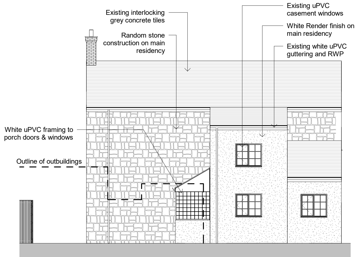
Existing Elevation 4 - Main Residency (No Change) 1 : 100
