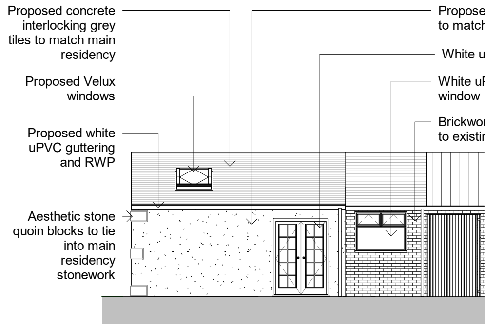
Proposed Elevation 1 1 : 100
