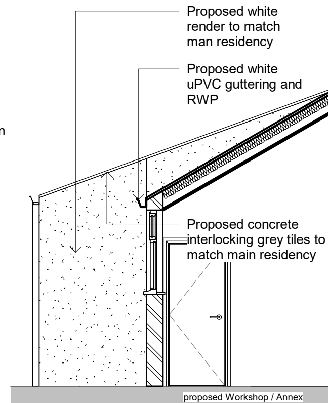
Proposed Elevation 5 1 : 50
