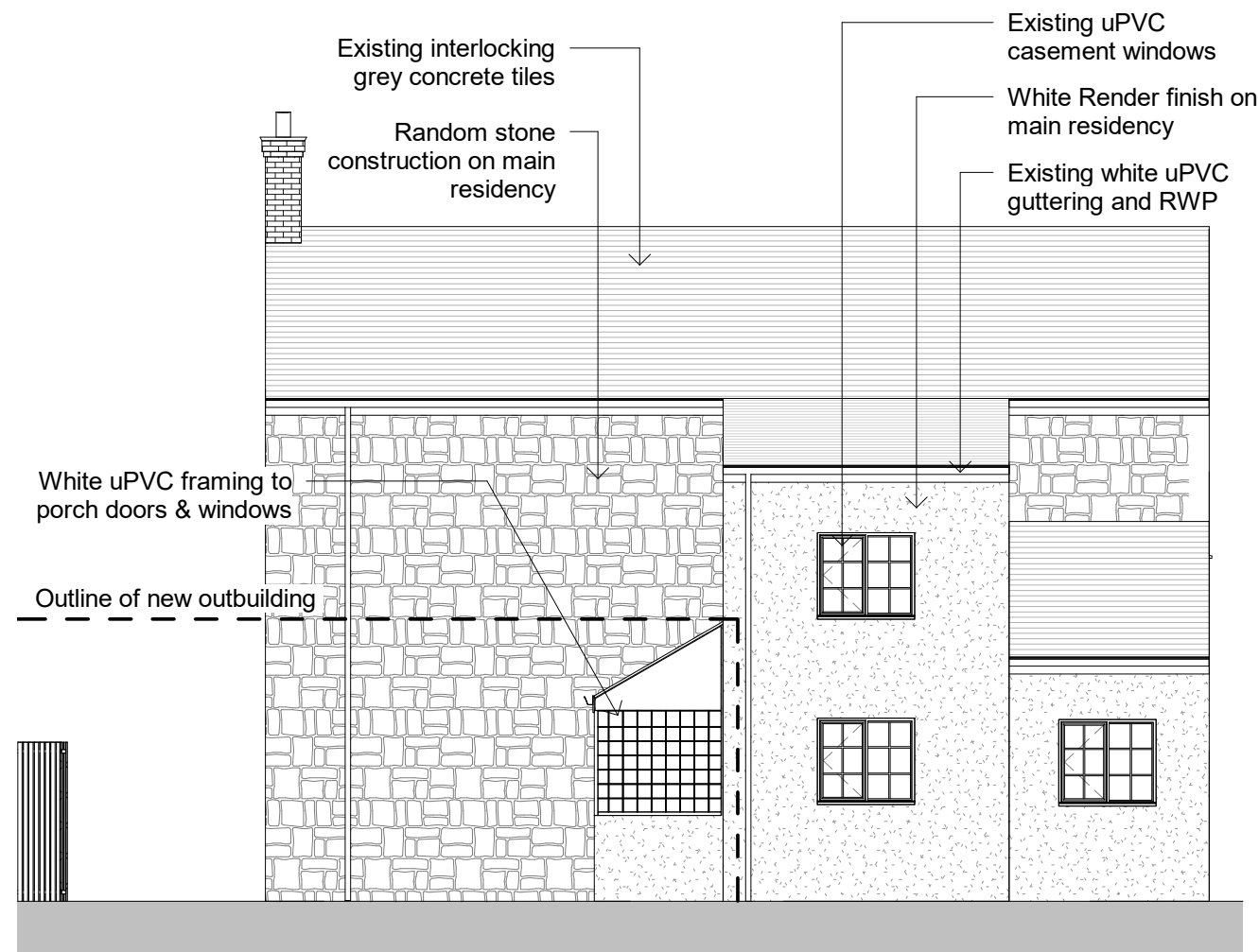
Proposed Elevation 4 - Main Residency (No Change) 1 : 100
