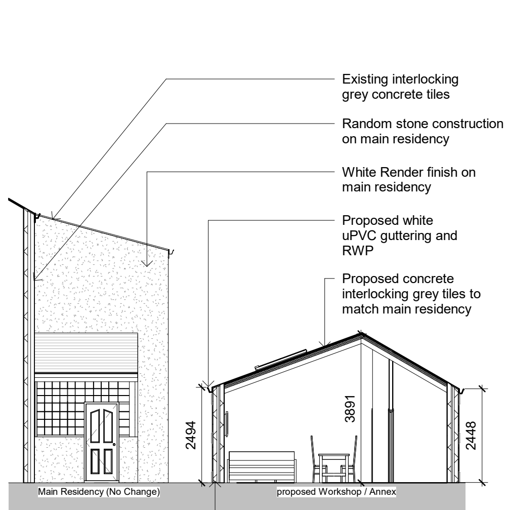
Proposed Section AA 1 : 100
