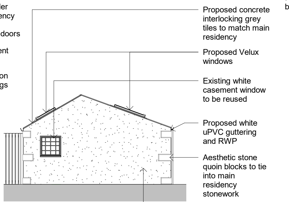
Proposed Elevation 2 1 : 100
