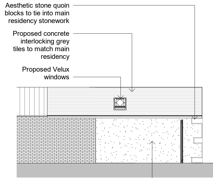
Proposed Elevation 3 1 : 100
