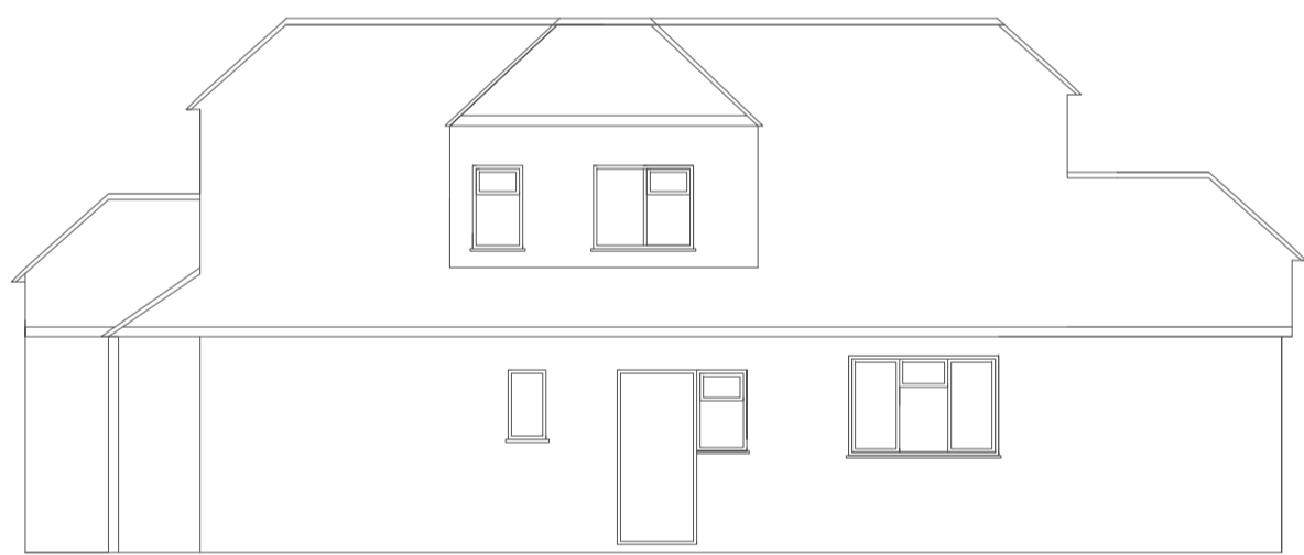
Existing Right Elevation
