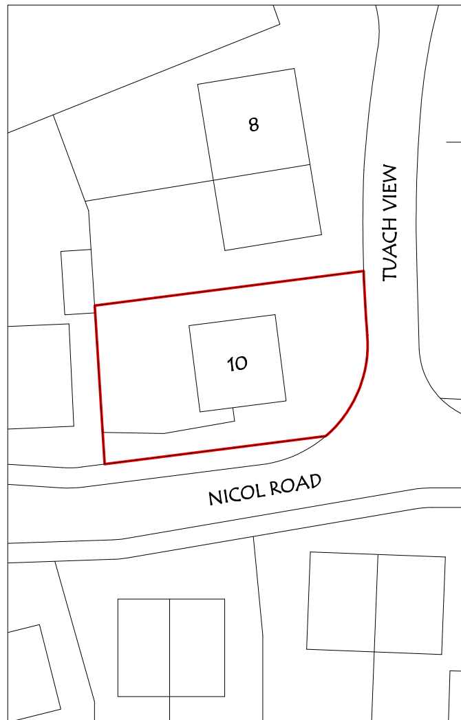
Site Plan Scale 1:500 @ A4
