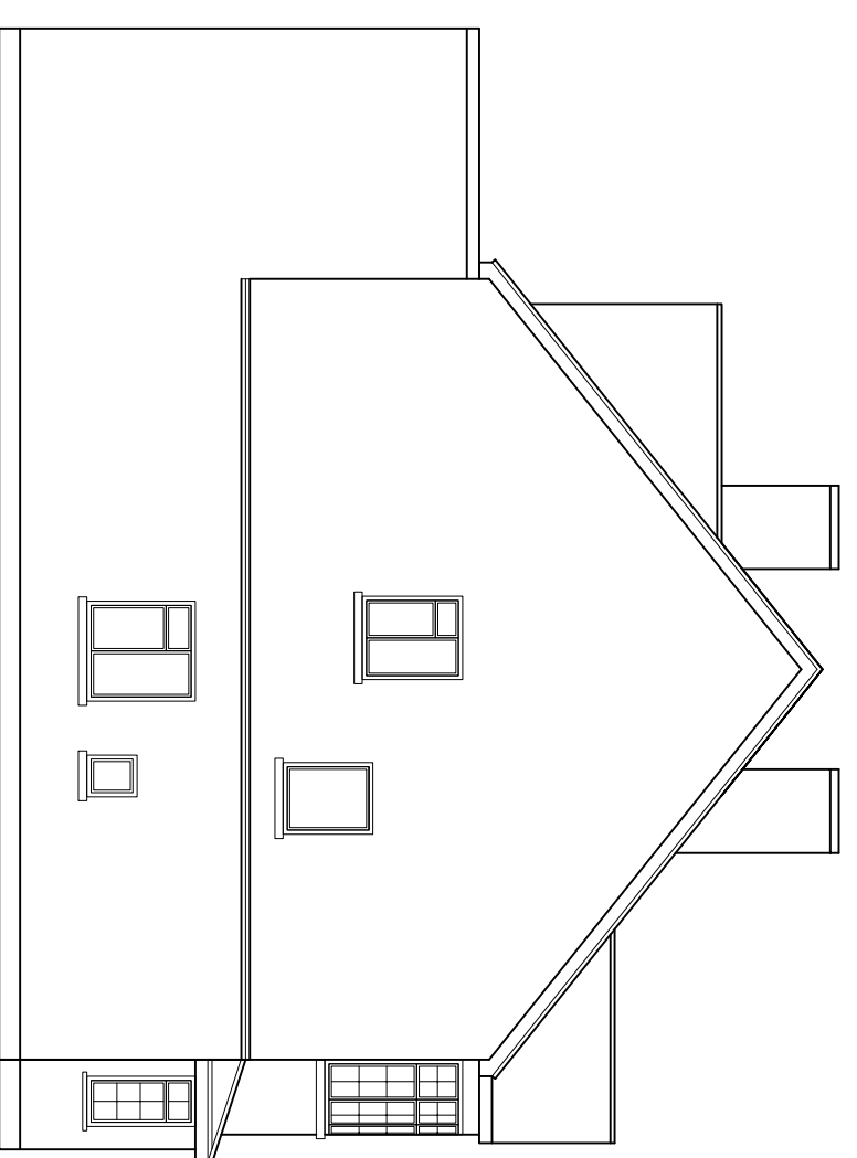
SIDE ELEVATION 2
