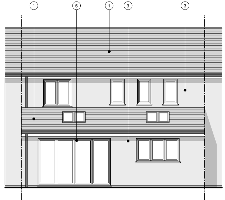
Proposed Rear Elevation - North
