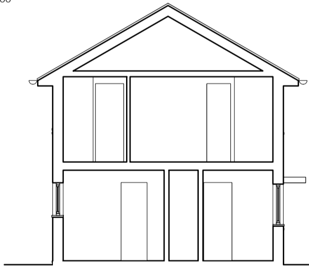
Existing Section
