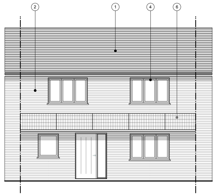
Proposed Front Elevation - South
