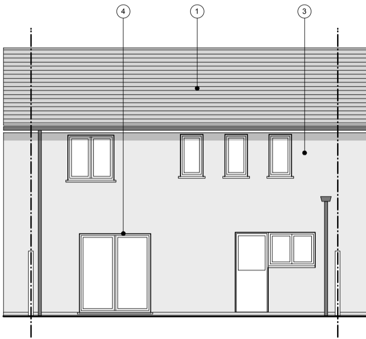
Existing Rear Elevation - North 1:100
