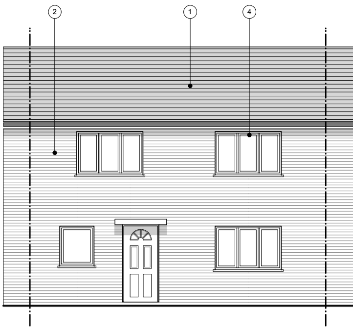
Existing Front Elevation - South 1:100
