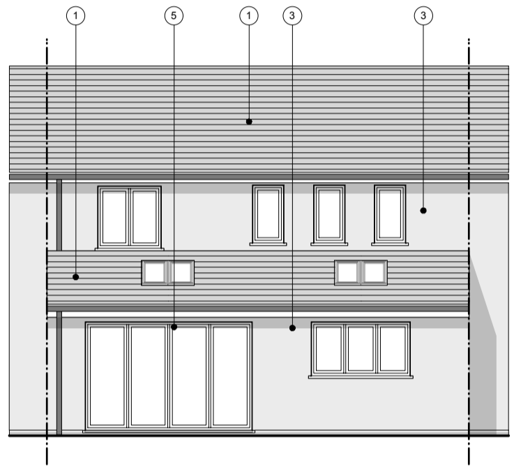
Proposed Rear Elevation - North 1:100
