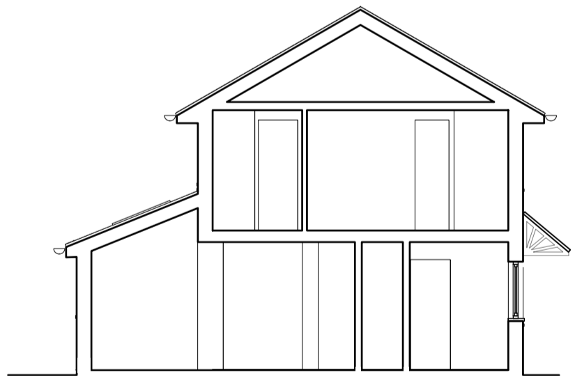
Proposed Section 1:100
