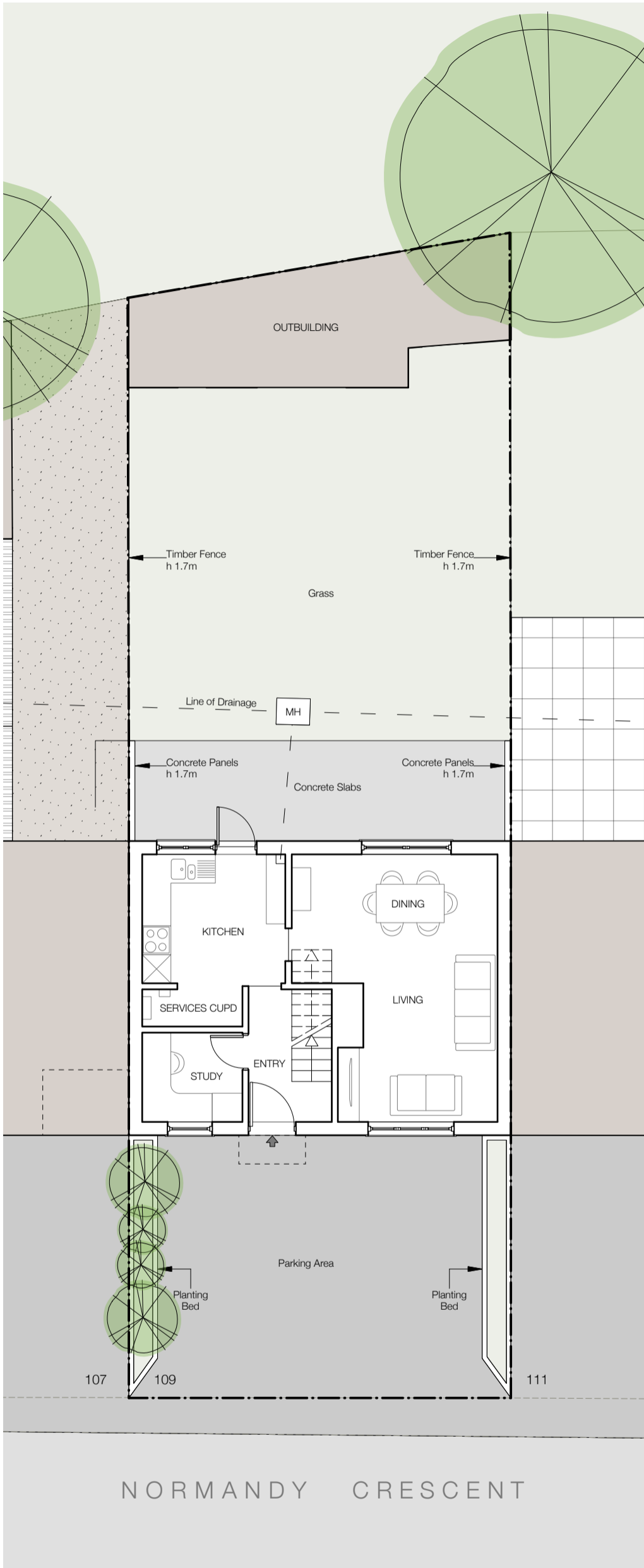
Existing Site and Ground Floor Plan 1:100
