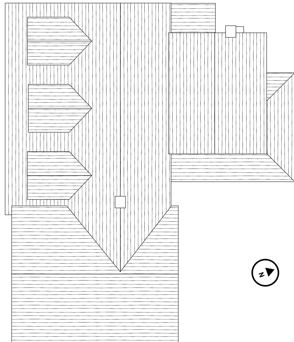
ROOF PLAN
