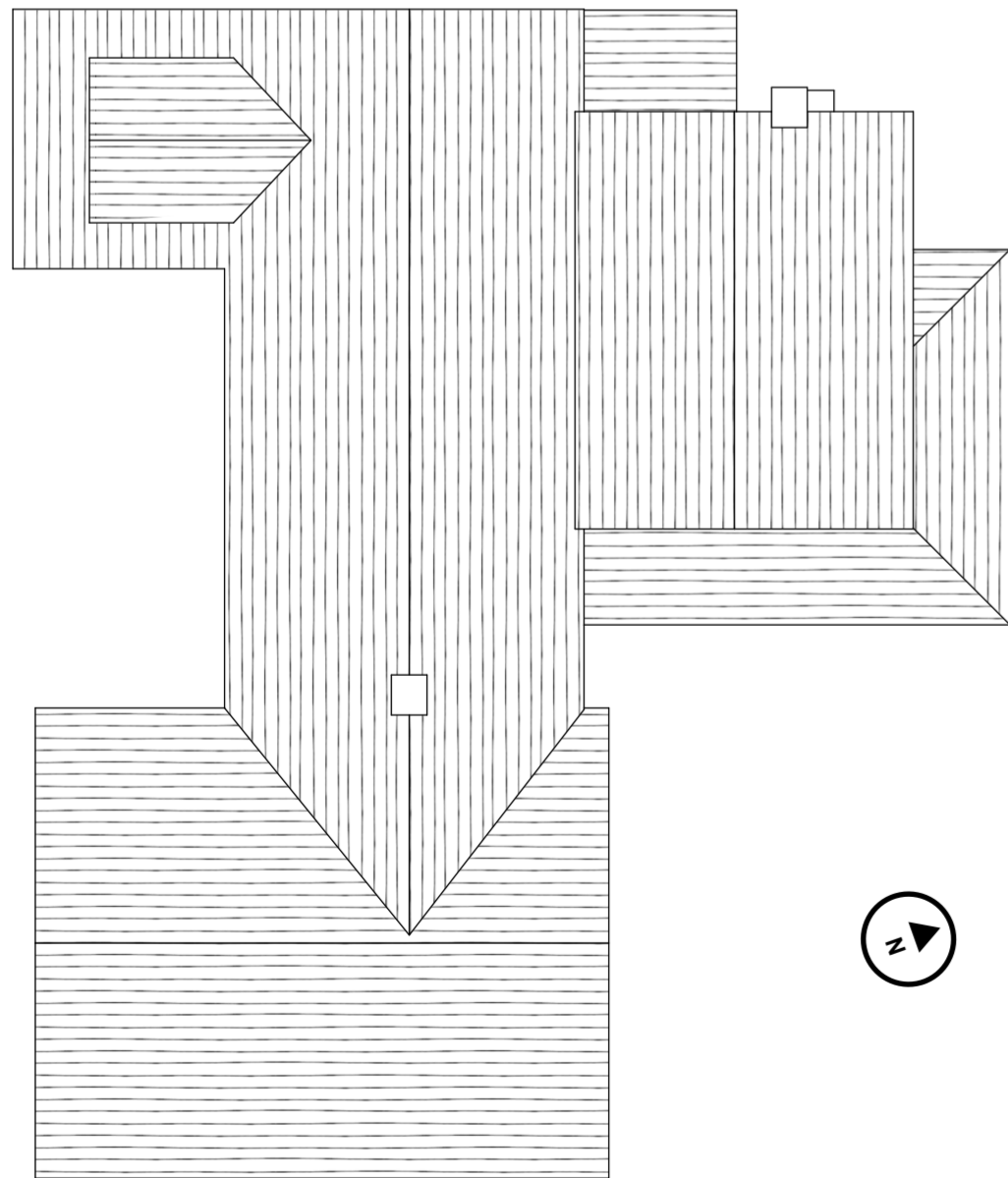
ROOF PLAN
