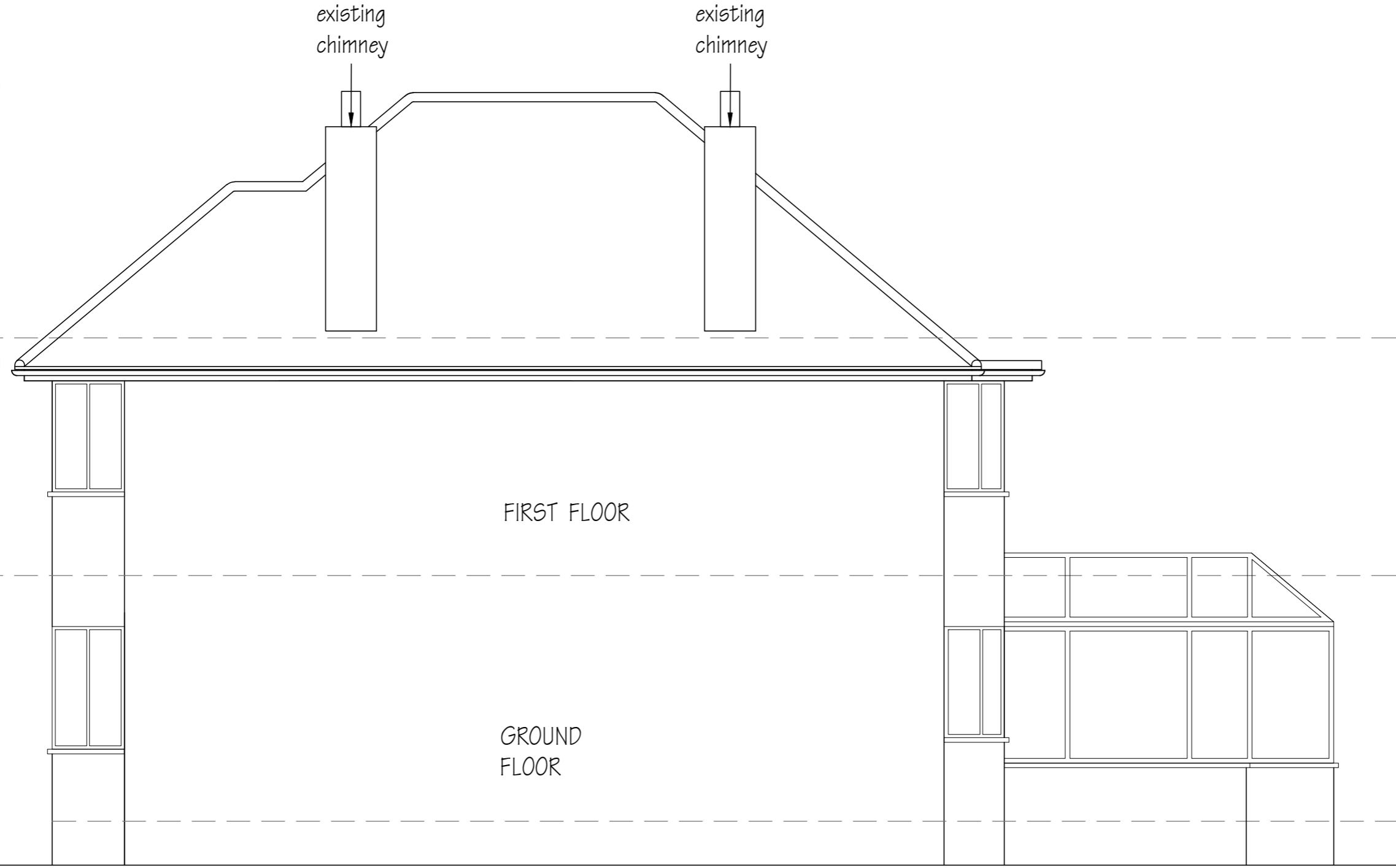
EXISTING WEST SIDE ELEVATION
