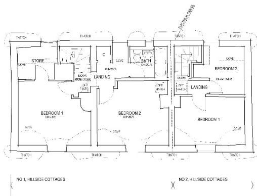
First Floor Plan – Existing
