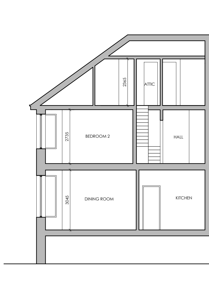
EXISTING SECTION A-A
