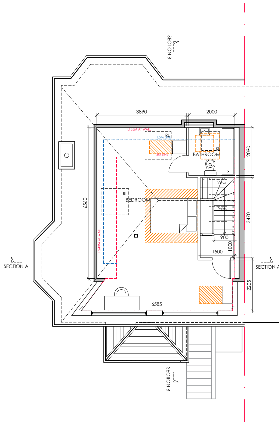
PROPOSED ATTIC FLOOR PLAN
