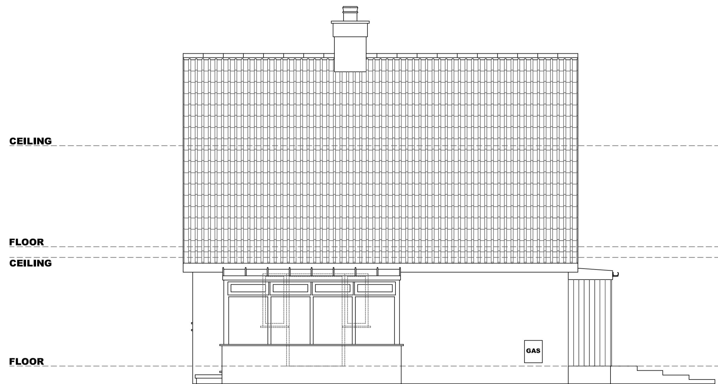
SOUTH ELEVATION AS EXISTING
