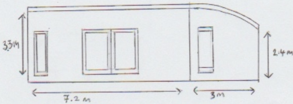
ELEVATION B / SOUTH EAST FACING
