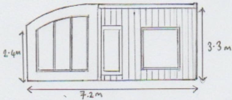
ELEVATION A / SOUTH WEST FACING
