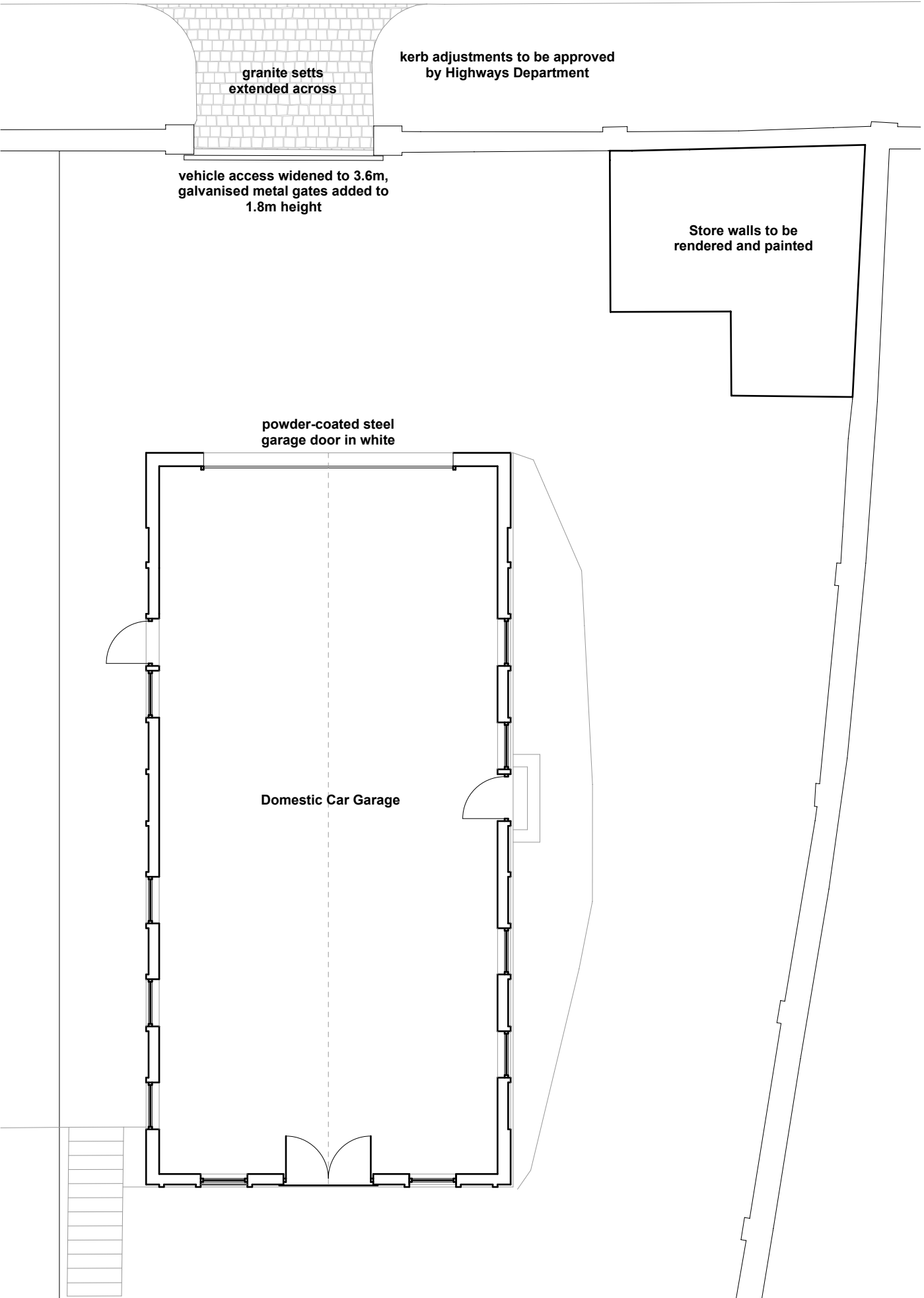
Proposed Floor Plan @ 1:100
