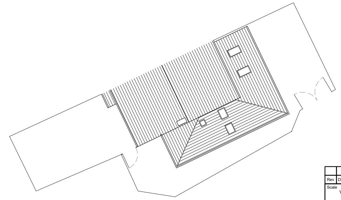
Proposed Site Plan 1:200@A3
