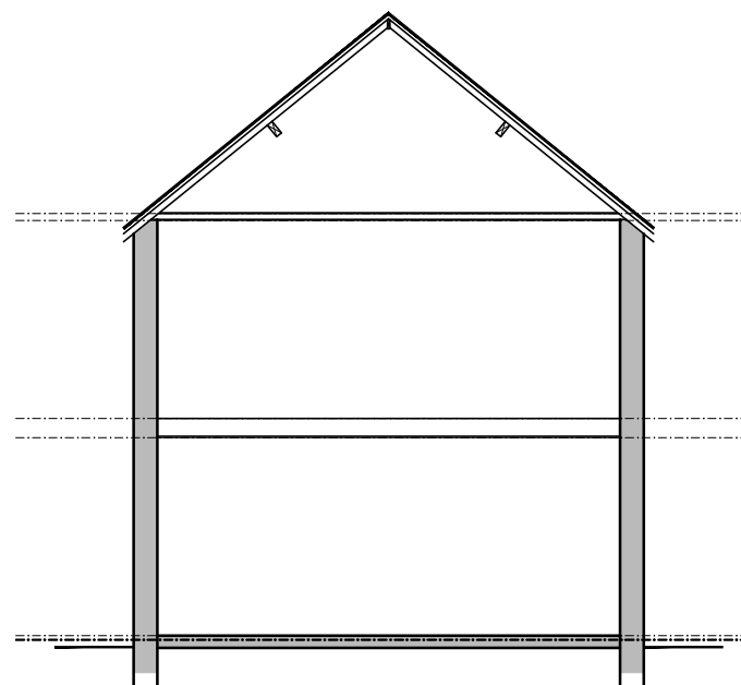
SIDE ELEVATION
