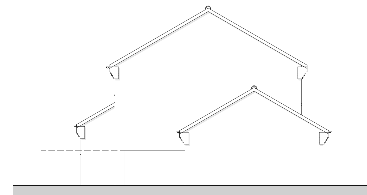
South-West Elevation
