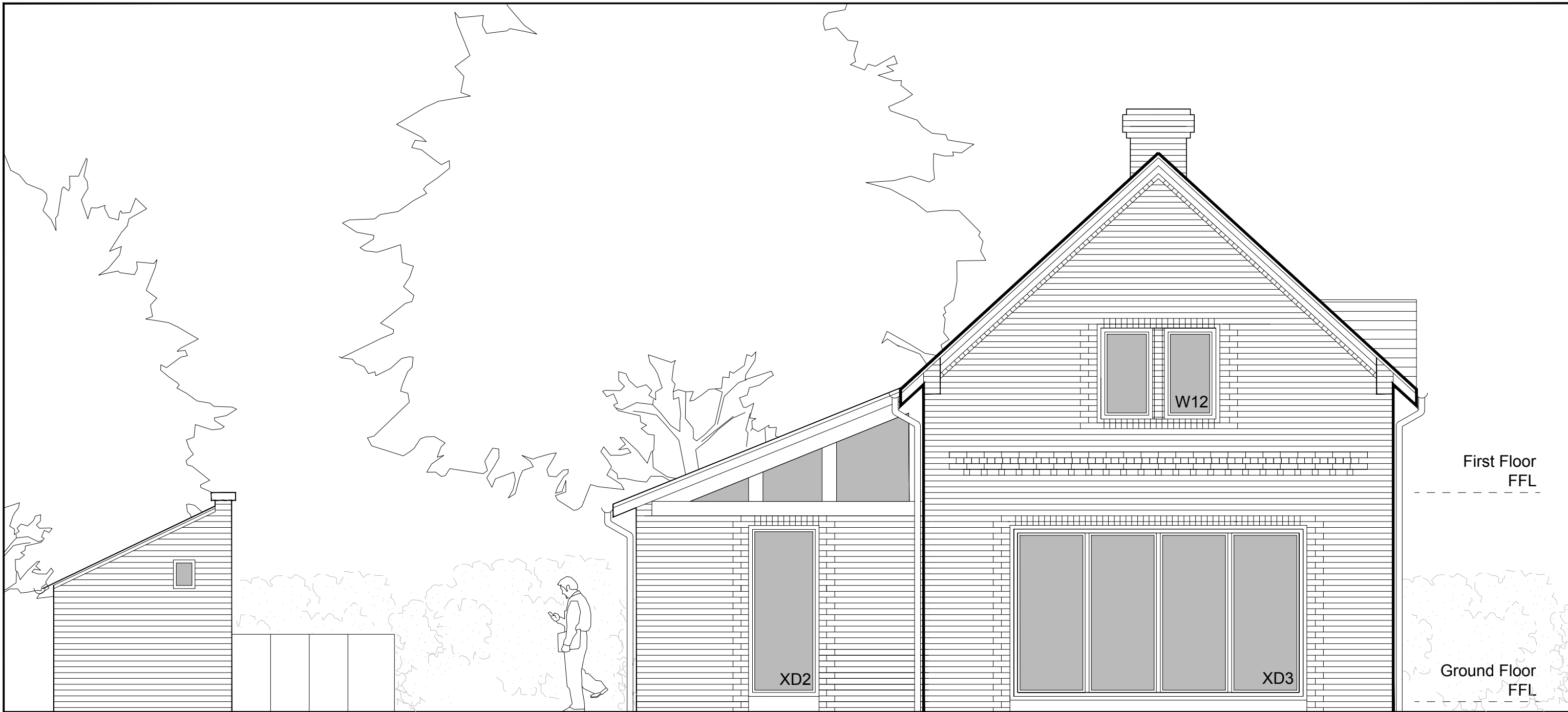
South West Elevation Scale 1:50
