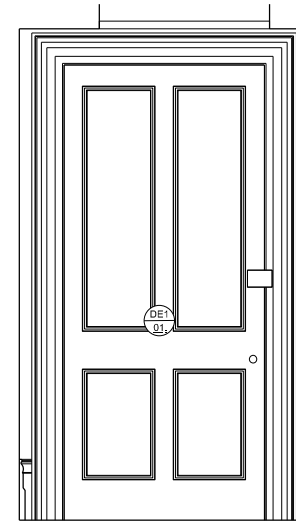
500_001 03 Elevation B 1:20
